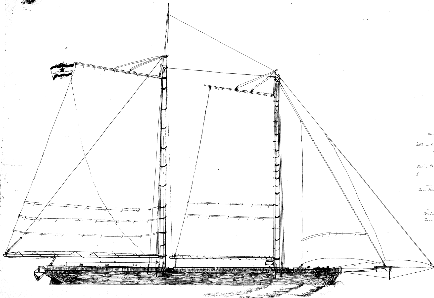
Schooner "Granada" - of the - Nicaraguan Navy. C. J. Fajeney, Commandr.
